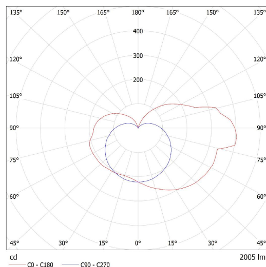
Lucis S5.L12.A450.0W ASTERION LED / LDC (Polar)
